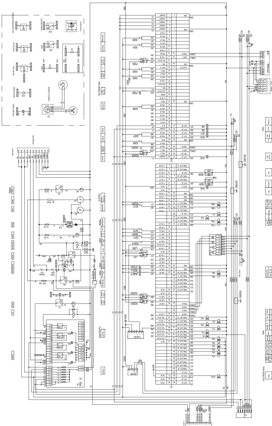
Electrical schematic of turntable, hydraulic generator(Deutz)
